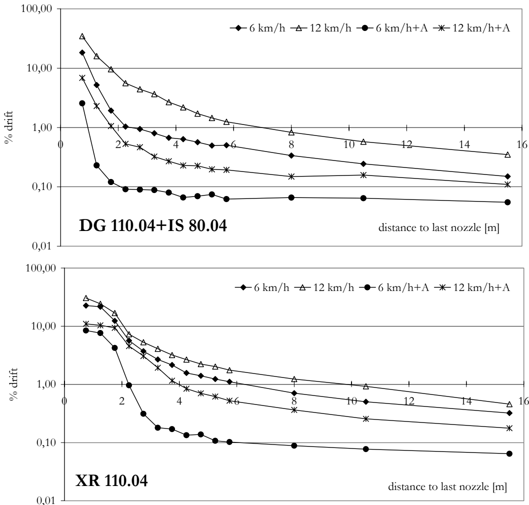
Figure 1. Spray drift deposition (% of volume application rate) next to a sprayed potato field using a conventional and an air-assisted sprayer at sprayer speeds of 6 km/h and 12 km/h with standard flat fan XR11004 and pre-orifice flat fan nozzles (DG11004) in combination with an end-nozzle (IS8004)
