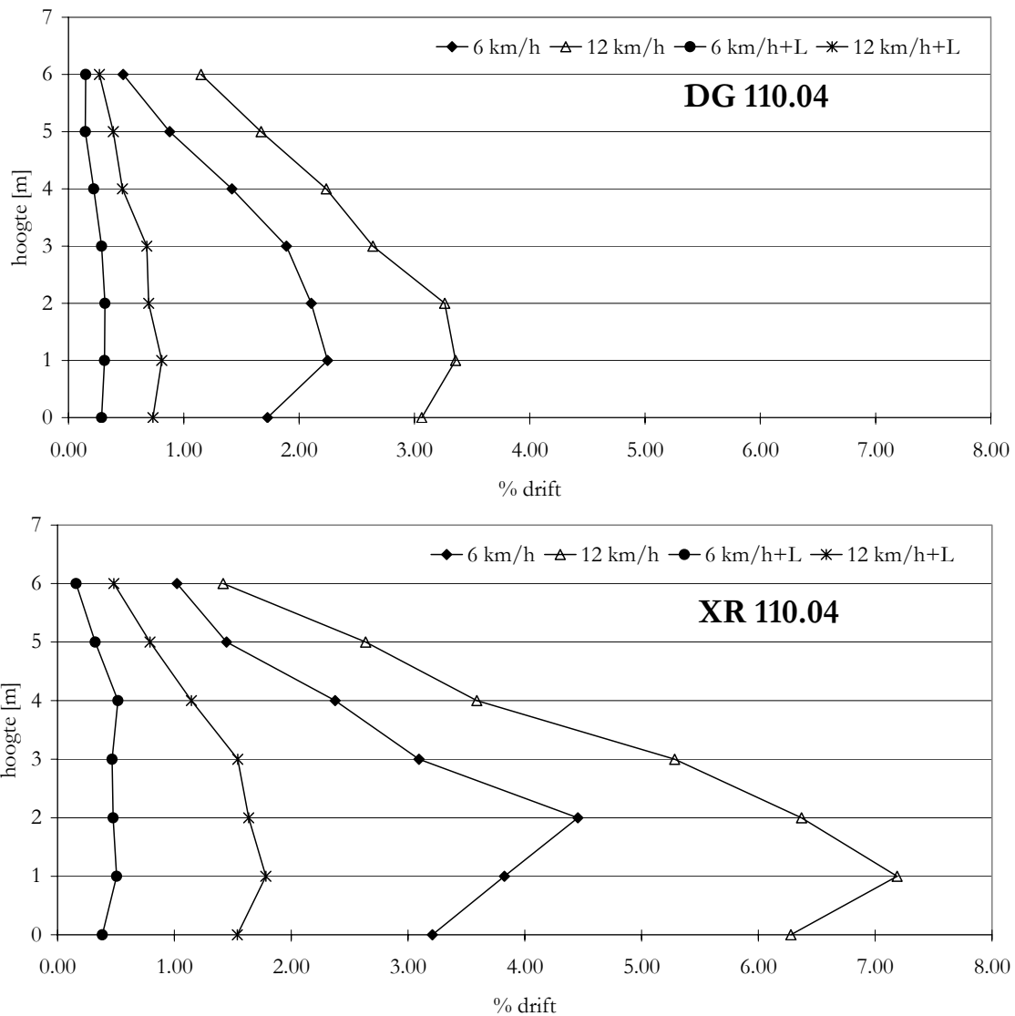
Figure 2. Airborne spray drift deposition (% of volume application rate) at 5.5 m distance from the last nozzle next to a sprayed potato field using a conventional and an air-assisted sprayer at sprayer speeds of 6 km/h and 12 km/h with standard flat fan XR11004 and pre-orifice flat fan nozzles (DG11004) in combination with an end-nozzle (IS8004)
